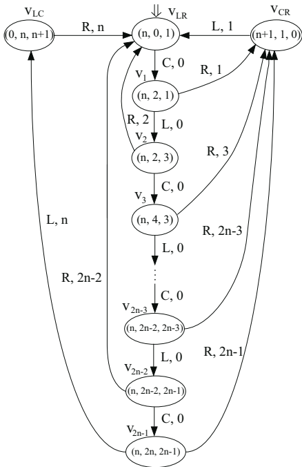
Fig. 3. Offset graph
