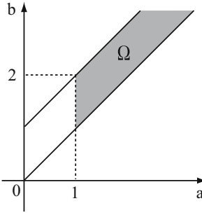
Fig. 5. Area \Omega
