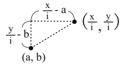
Fig. 12. Lines 40-47
